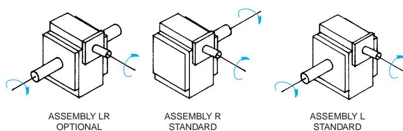
The input shaft may be driven in either direction.
