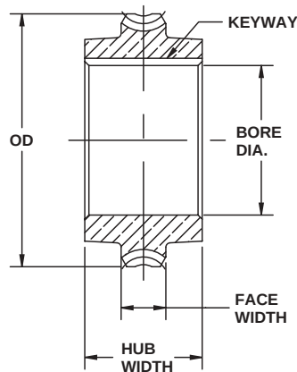
HOLLOW SHAFT GEAR
