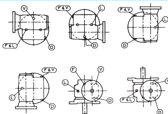
Standard Mounting Positions & Plug Locations
