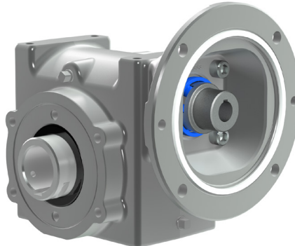
HOLLOW OUTPUT
